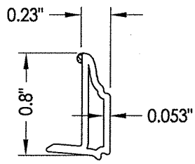
3 GLAZING BEAD
