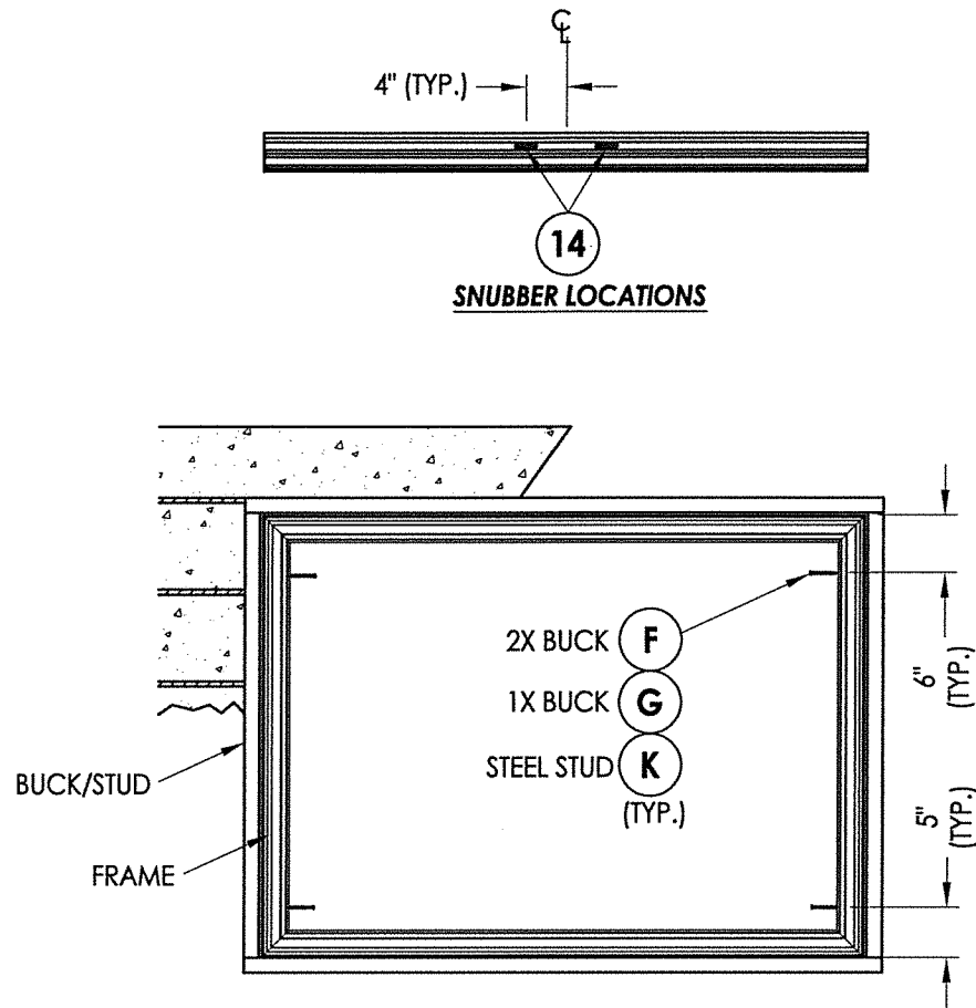
FRAME ANCHORING
