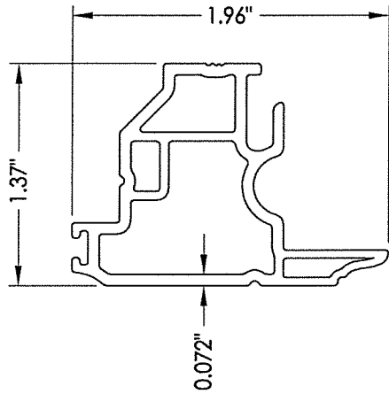
2 SASH
